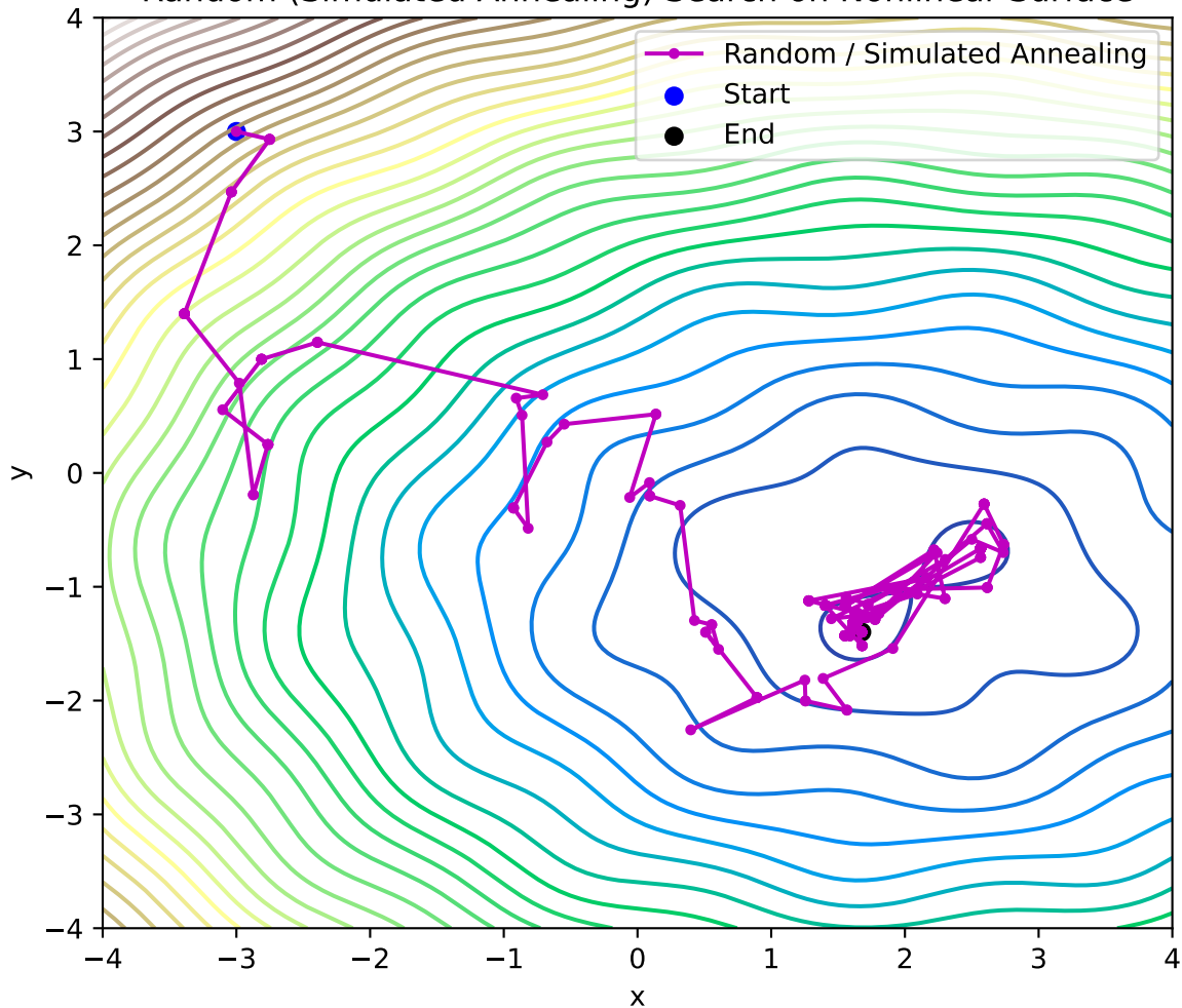
Random (Simulated Annealing) Search on Nonlinear Surface
